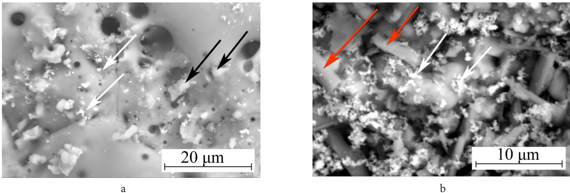
Fig. S1. (Color online) SEM images of the coating surface for Zn-TCP (a), and Zn-Wol (b).
