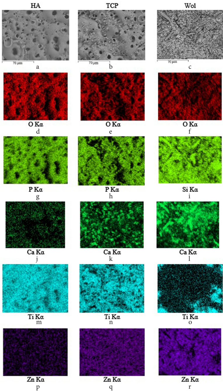
Fig. S2. (Color online) SEM images of coatings (a – c) and elements distribution maps (d – r).
