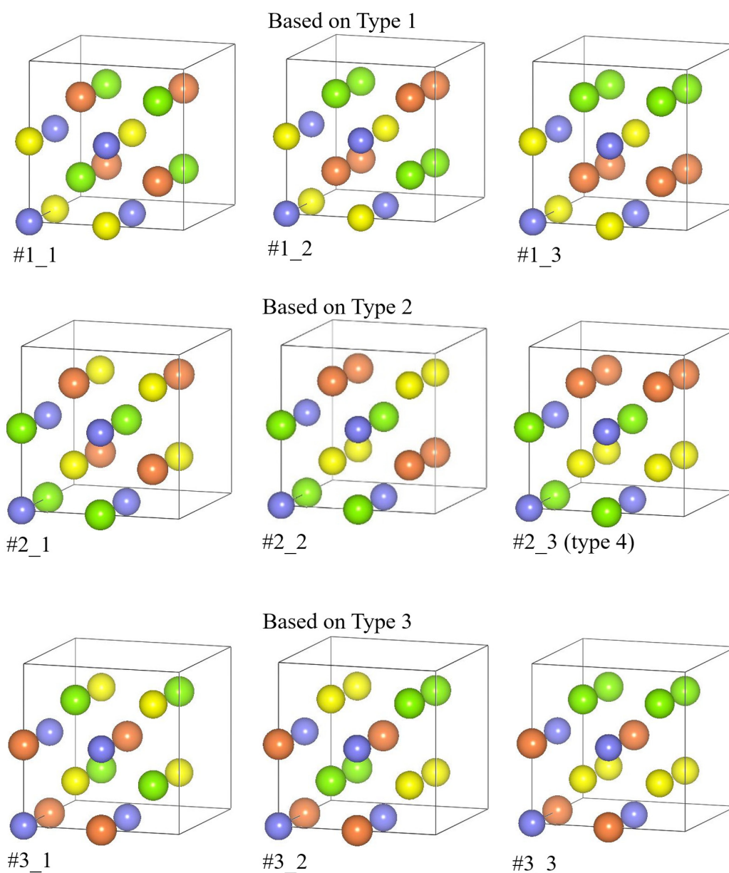
Fig. S1. (Color online) All considered atomic configurations for FeMnVGe.
