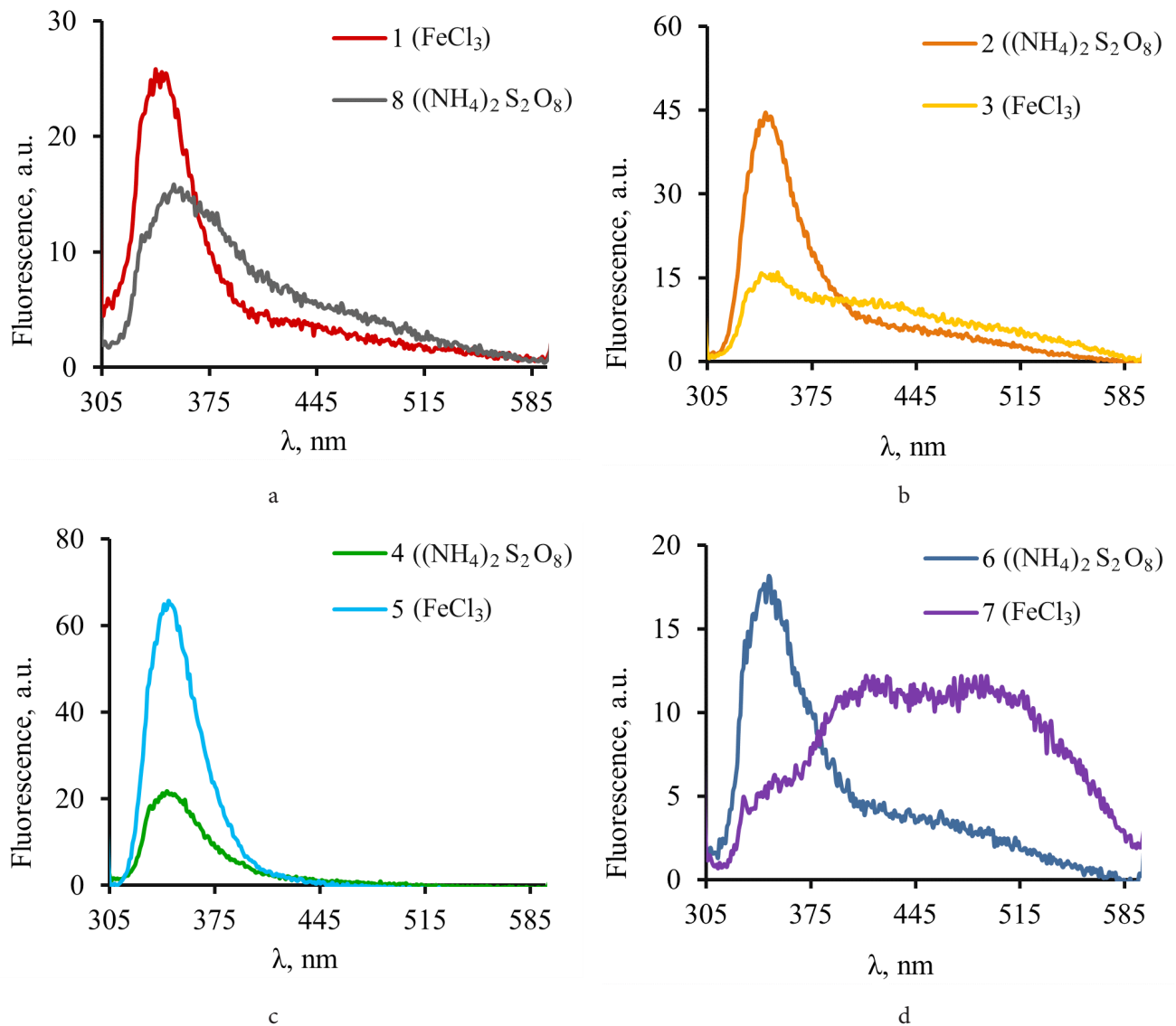
Fig. 1S. (Color online) Fluorescence spectra of samples 1 and 8 (a), 2 and 3 (b), 4 and 5 (c), 6 and 7 (d) in DMSO solution ( 1.25 \times 10^{-3} g/l).
