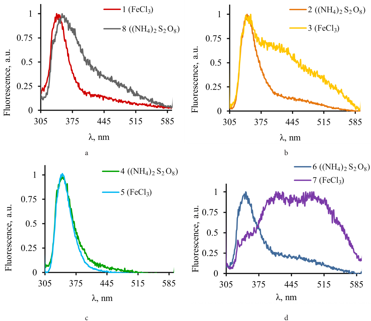
Fig. 25. (Color online) Normalized fluorescence spectra of samples 1–8 in DMSO solution ( 1.25 \times 10^{-3} g/l).
