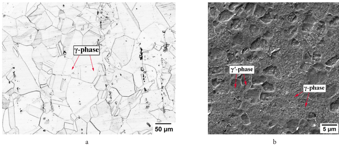
Fig. S1. Initial microstructure of superalloys: EK61 (a), EP975 (b).
