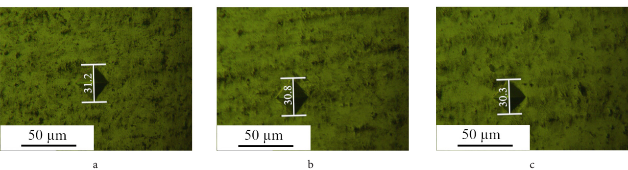
Fig. S2. (Color online) Vickers microhardness indent marks of commercially pure titanium under different electric potentials (without applying of electric potential (a), 0.5 V (b), 1 V (c)).
