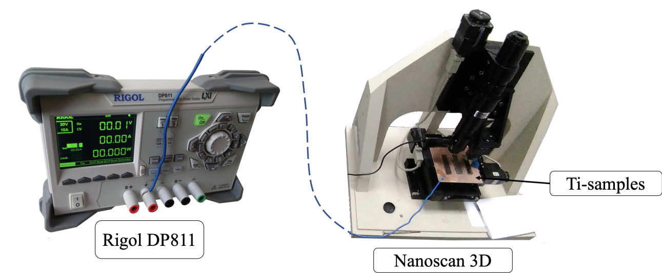
Fig. S1. (Color online) Wiring diagram of the electric potential supply with Ti-samples when testing the elastic modulus.
