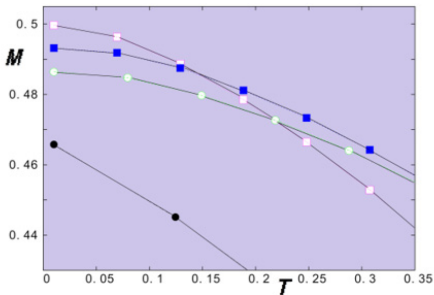
Fig. S2. Zoom at low T to show magnetization cross-overs.
