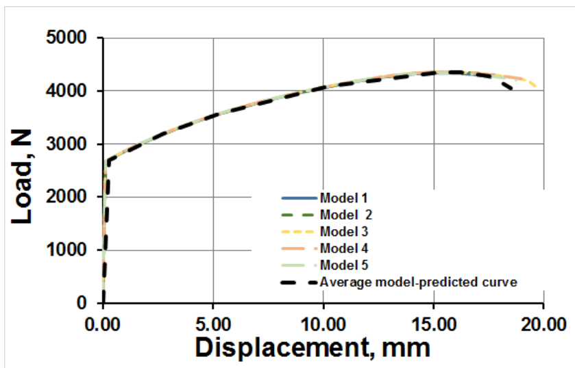
Fig. 55. The average model-predicted curve for nonhomogeneous specimens B.
