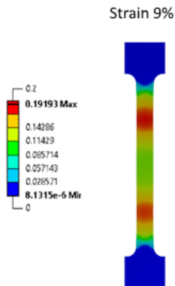
Fig. 56. Equivalent total strain at specimen elongation by 9%.
