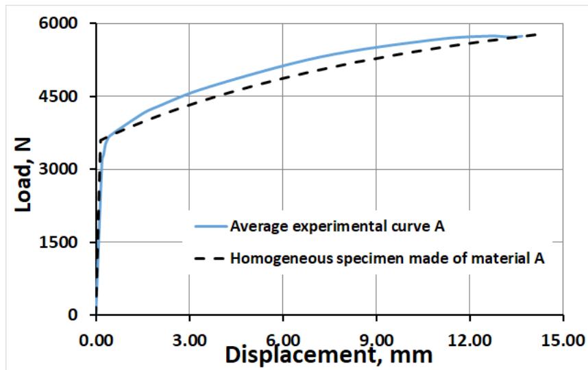
Fig. S1. Comparison of modeling results of a homogeneous specimen from material A with the average experimental curve.
