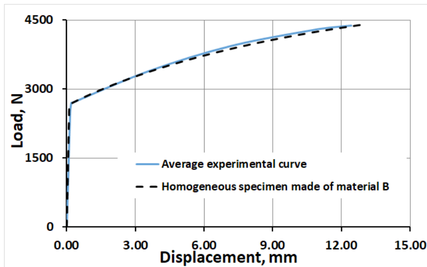
Fig. S2. Comparison of modeling results of a homogeneous specimen from material B with the average experimental curve.
