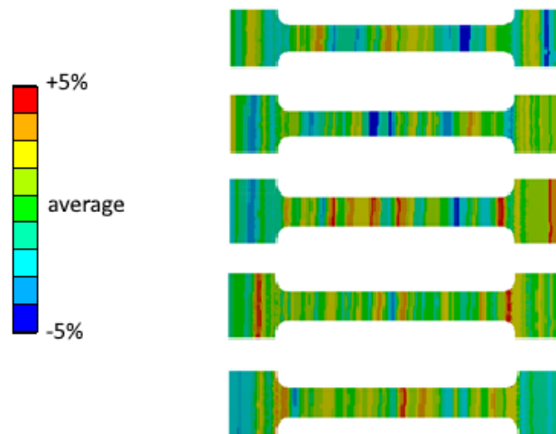
Fig. S3. Lengthwise property variation for specimens A.
