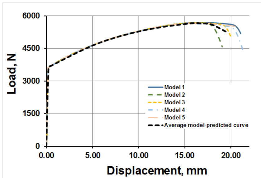
Fig. 54. The average model-predicted curve for nonhomogeneous specimens A.
